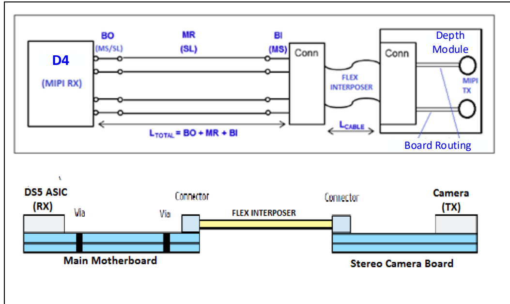
Figure 8-6. Stereo Depth Transmit - Vision Processor D4 Receive
