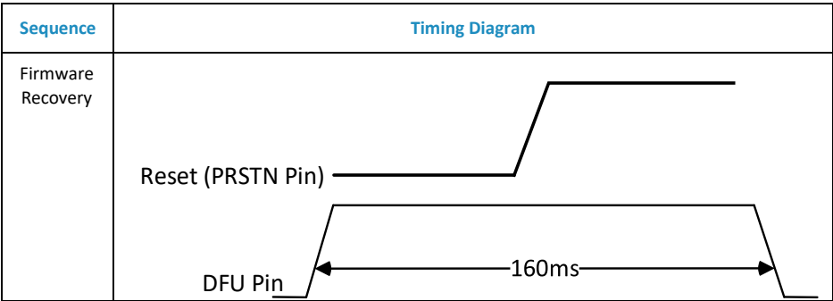
Figure 7-19. Firmware Recovery Sequence
